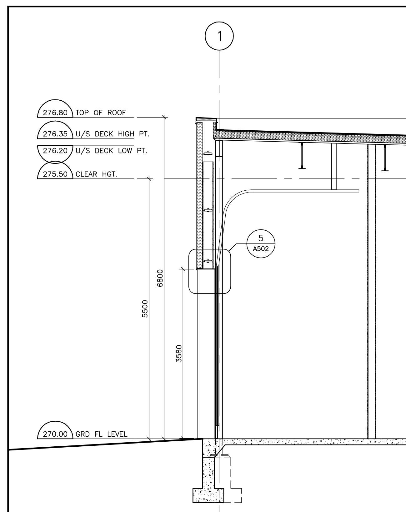
2 SECTION THROUGH O/H DOOR 1:50
