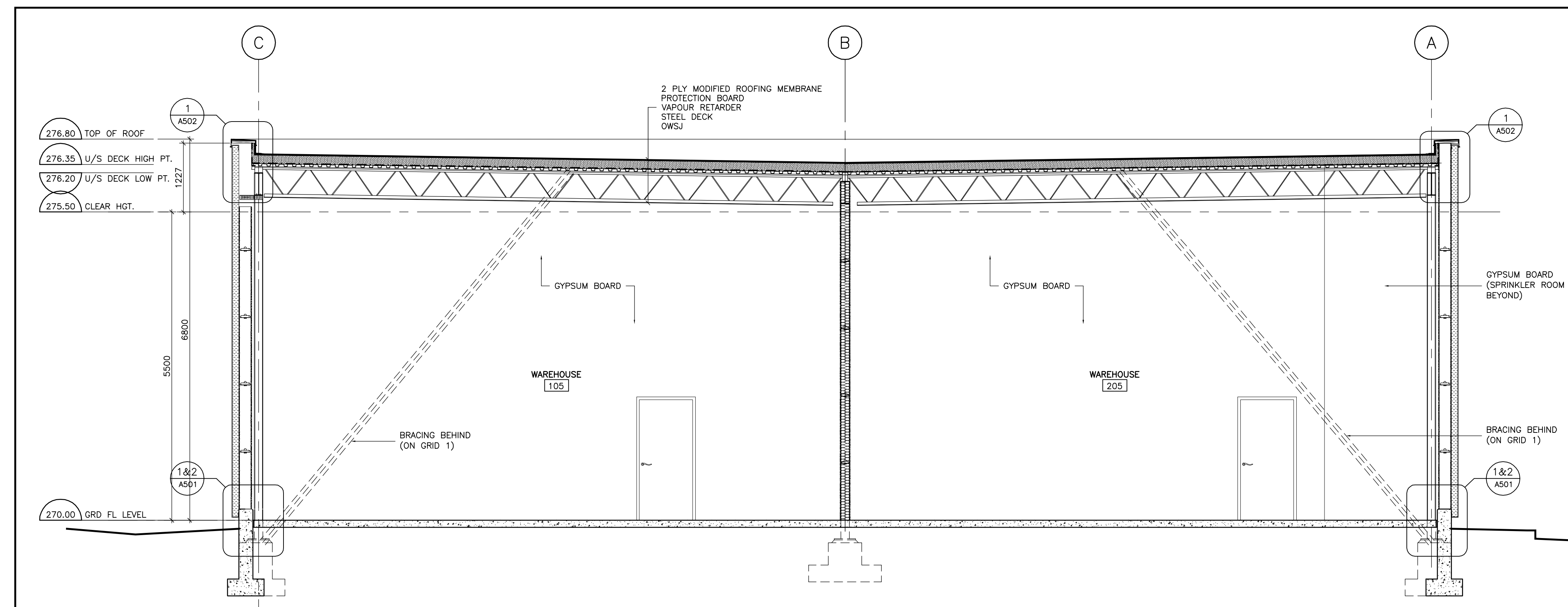
1 CROSS SECTION 1:50
