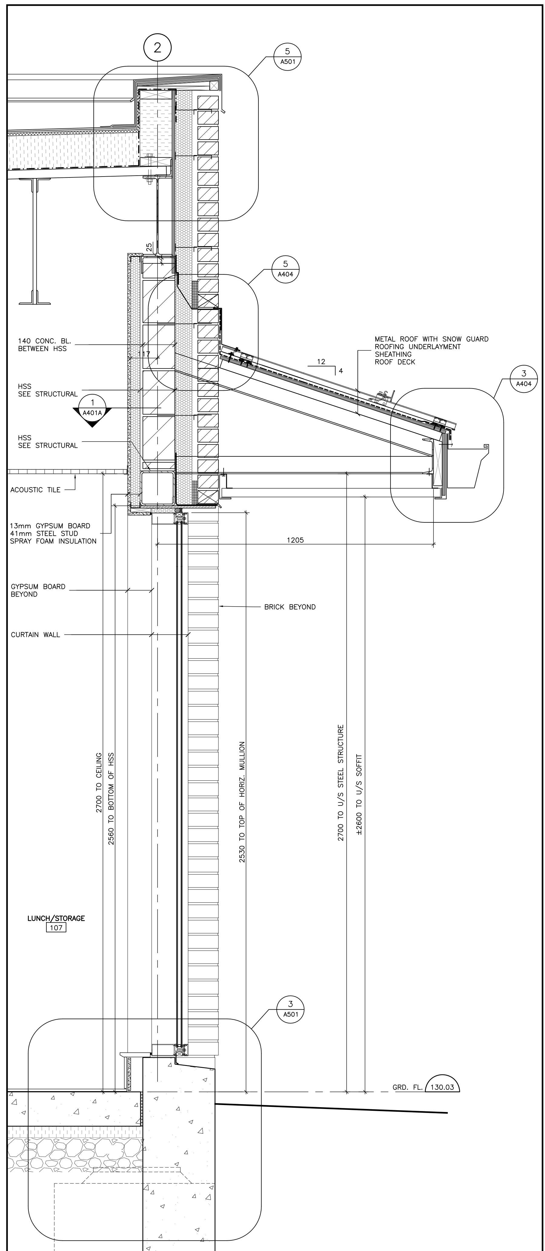
2 SECTION-CANOPY AT LUNCH/STORAGE 107 1:10
