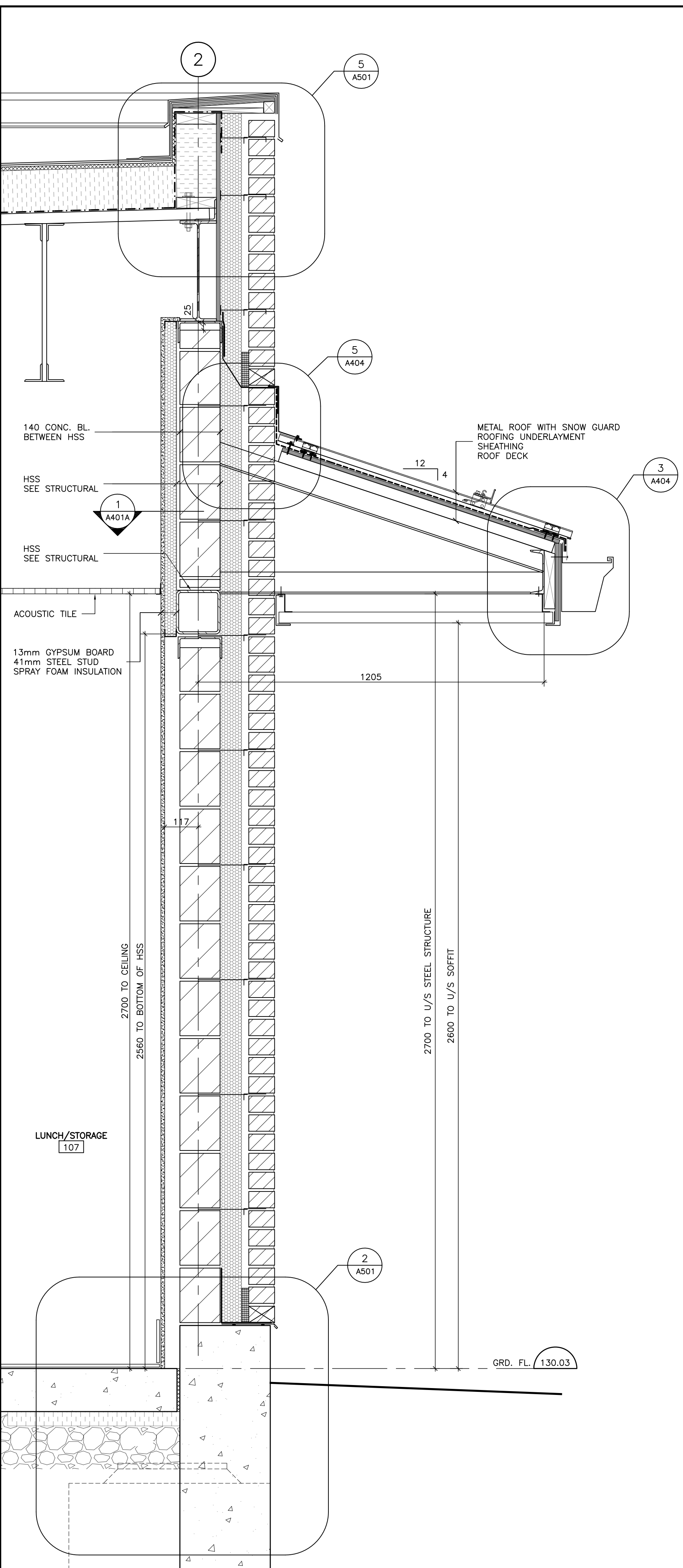
1 SECTION-CANOPY AT LUNCH/STORAGE 107 1:10
