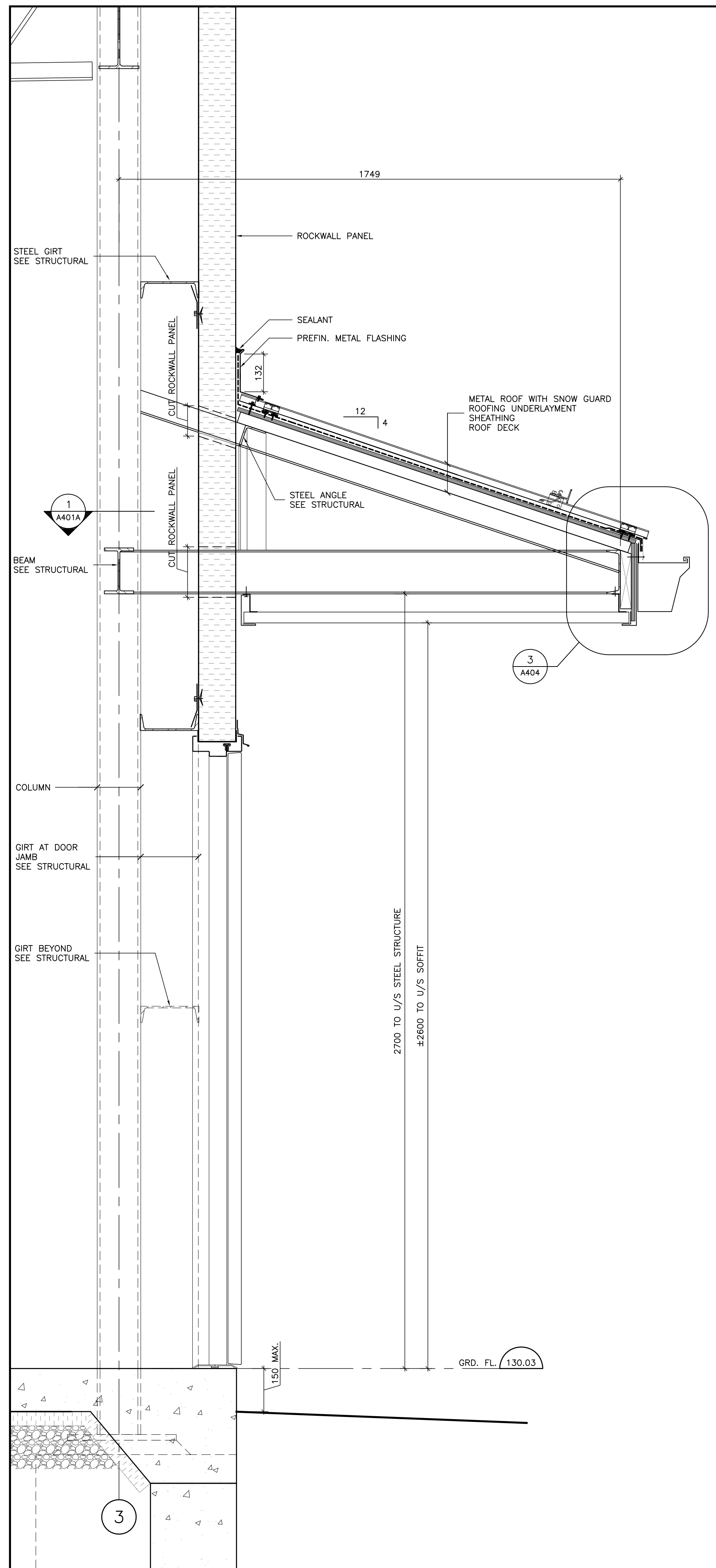
3 SECTION-CANOPY WAREHOUSE 1:10
