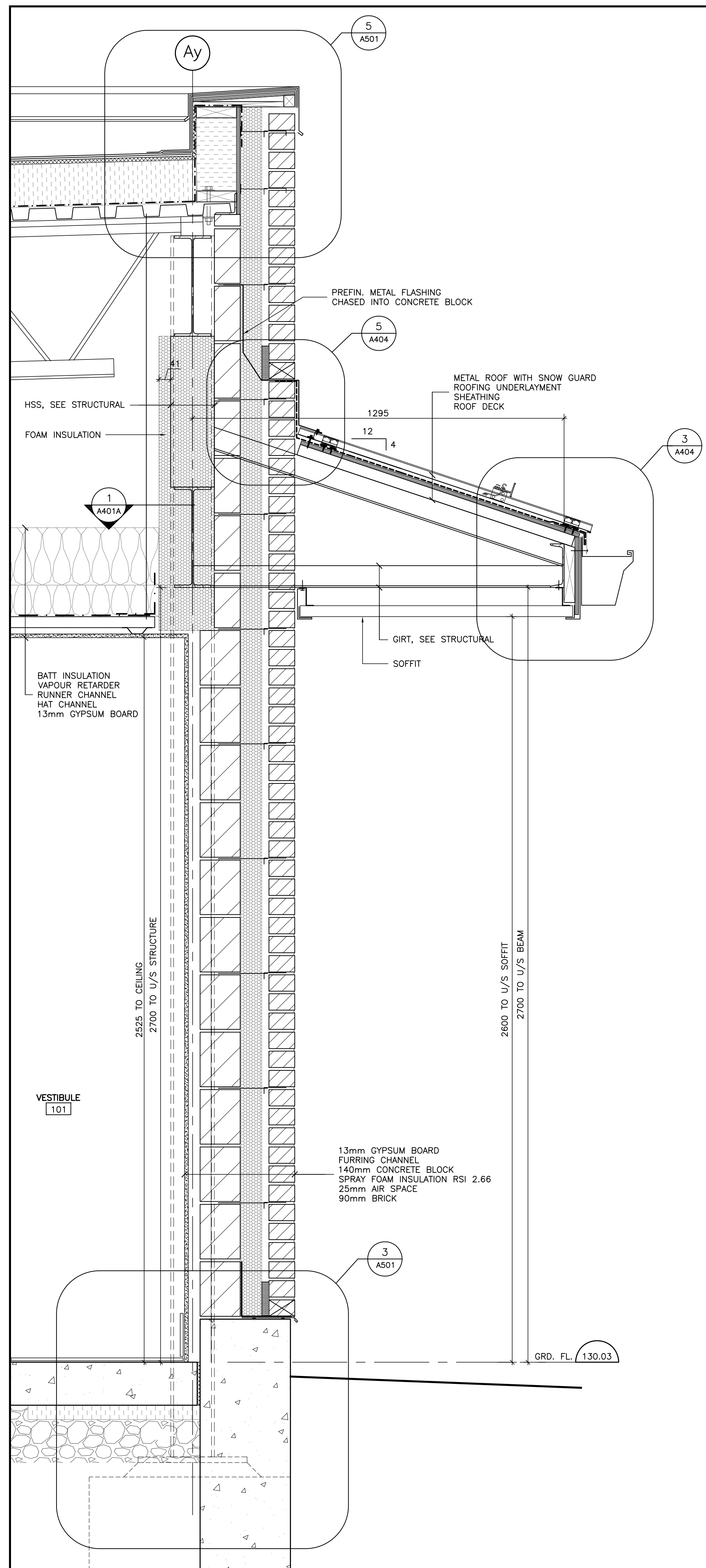
2 SECTION-CANOPY AT VESTIBULE 1:10
