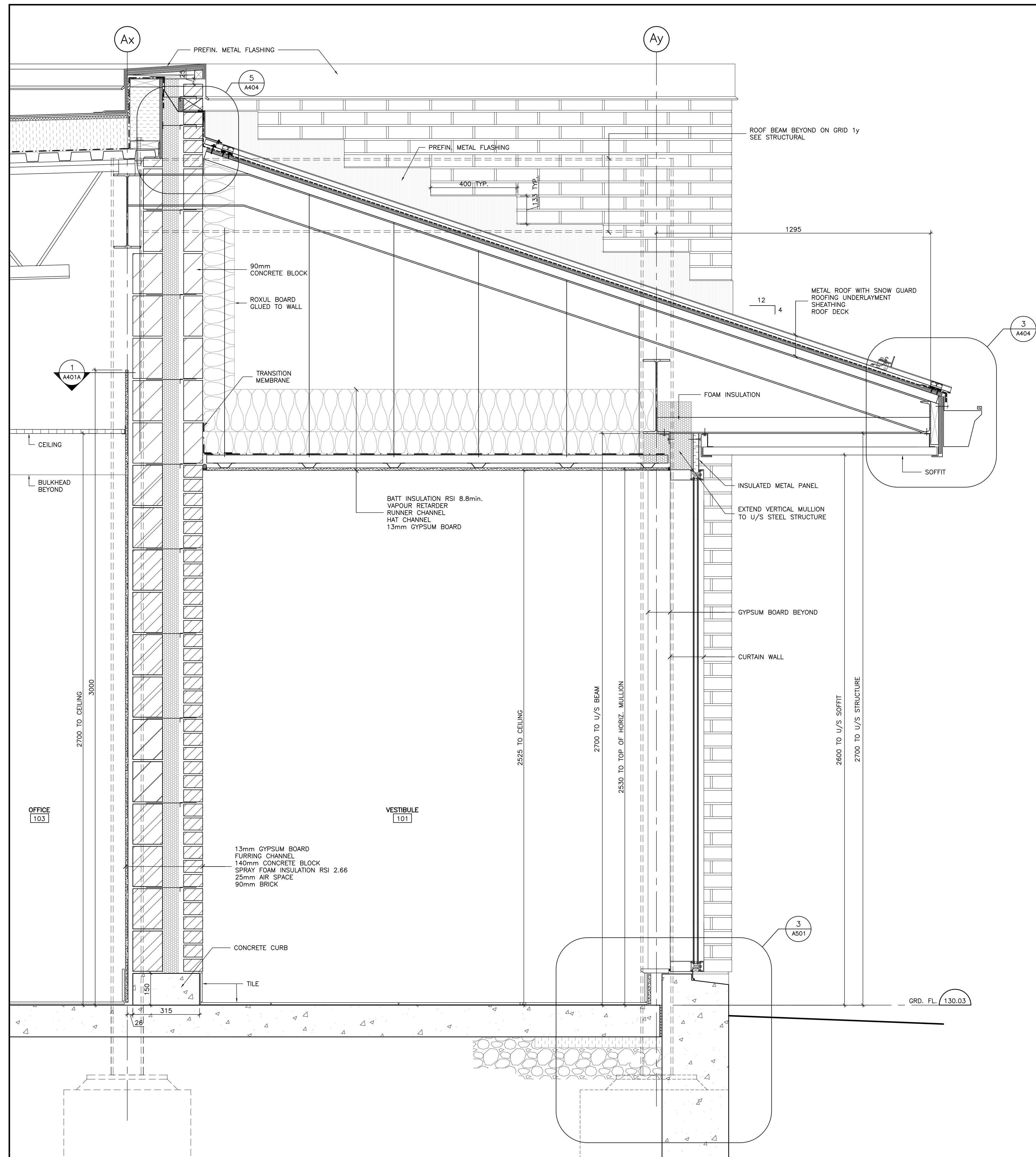
1 SECTION-CANOPY AT VESTIBULE 1:10
