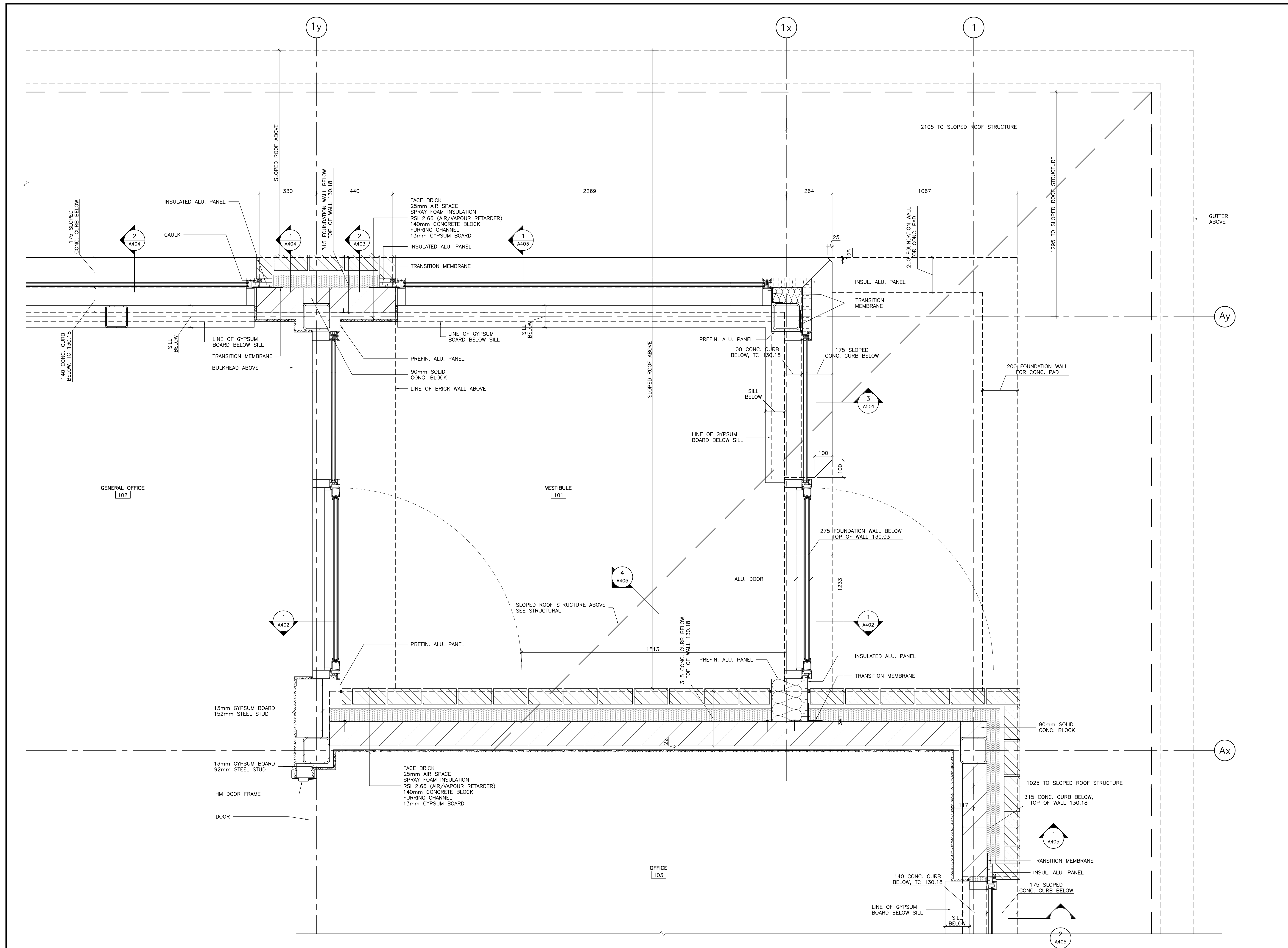
1 PLAN DETAIL - MAIN ENTRANCE 1:10
